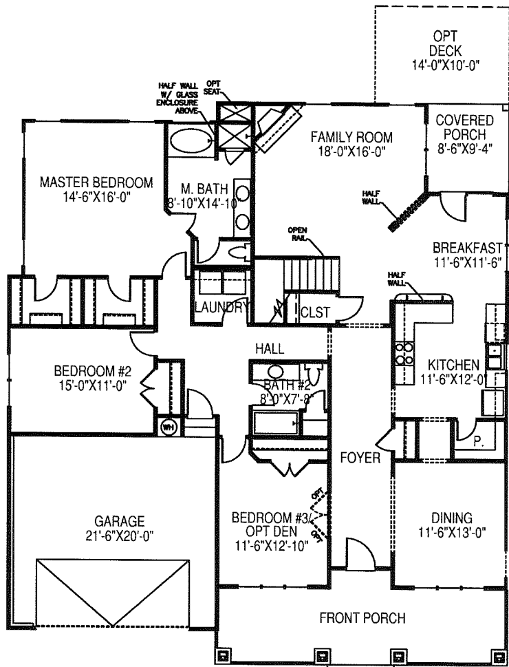
Buckingham First Floor Plan-Craftsman
