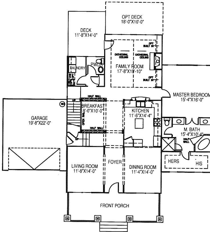
FRONT Montreat First Floor Plan-Craftsman
