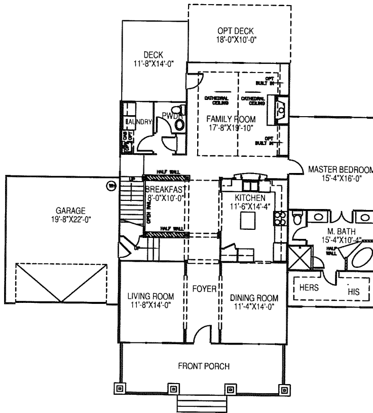
FRONT Montreat First Floor Plan-Lodge
