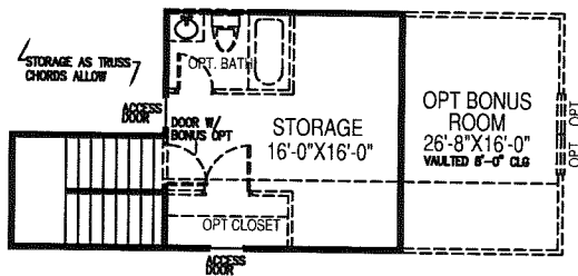
Nantahala Second Floor Plan-Cottage
