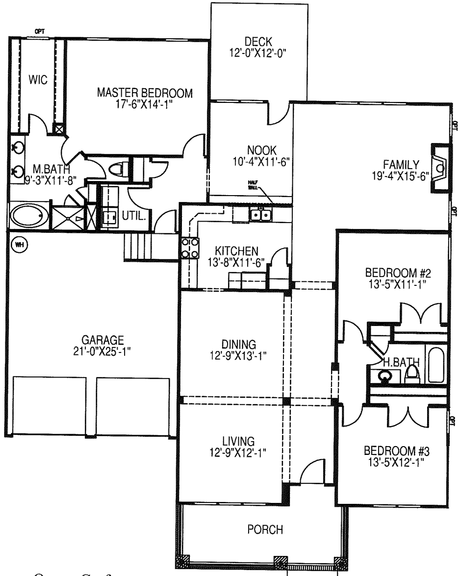
Ocoee Craftsman Main Floor Plan
