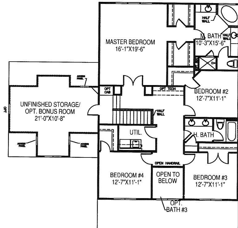
Pacolet Craftsman Second Floor Plan
