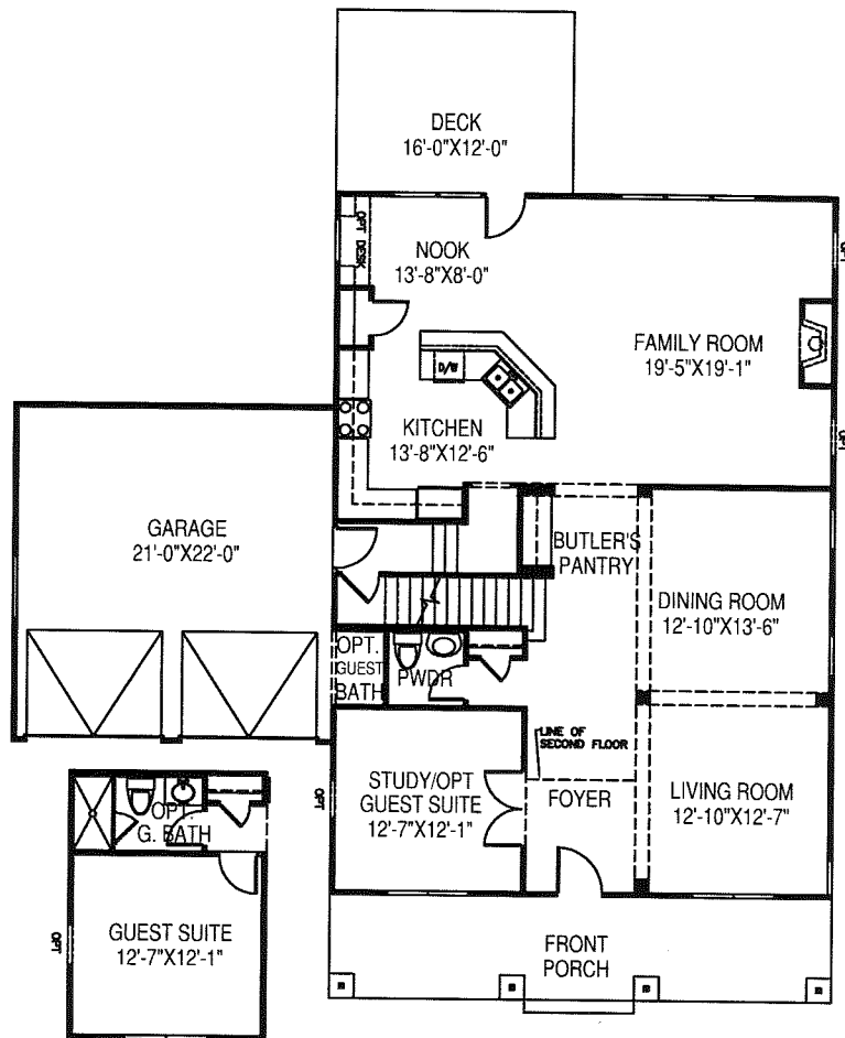
Pacolet-Craftsman First Floor Plan FRONT
