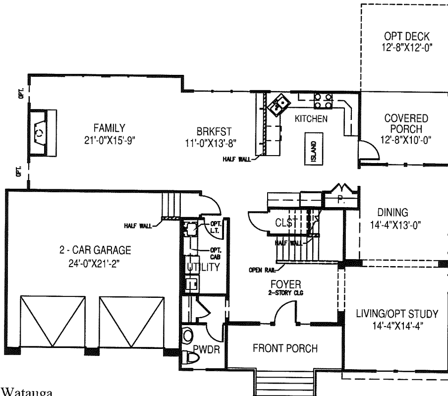
Watauga First Floor Plan-French
