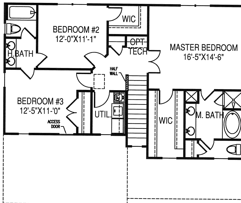
Cumberland Classical Second Floor Plan
