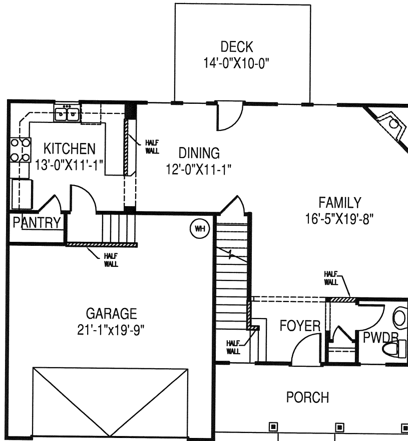
Cumberland Classical First Floor Plan
