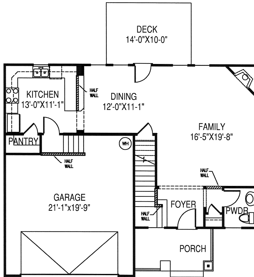
Cumberland Craftsman First Floor Plan
