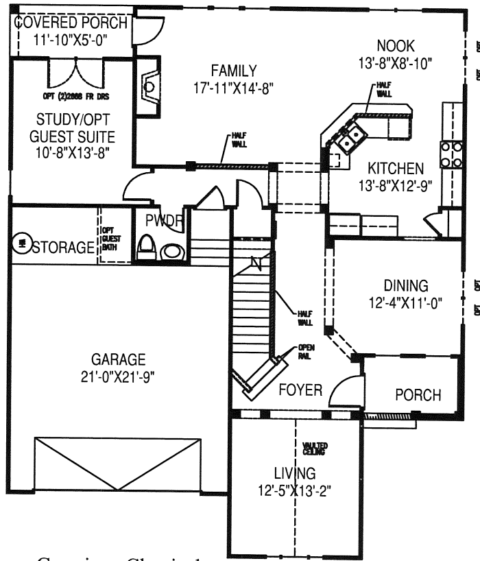
Gunnison Classical First Floor Plan
