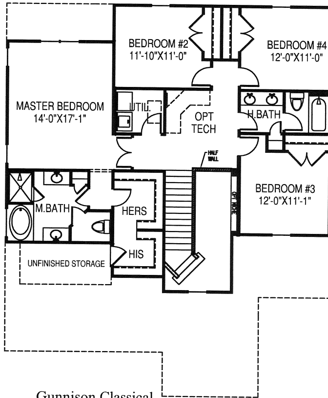
Gunnison Classical Second Floor Plan
