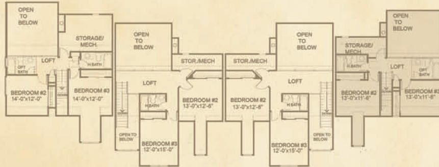
UPPER LEVEL
